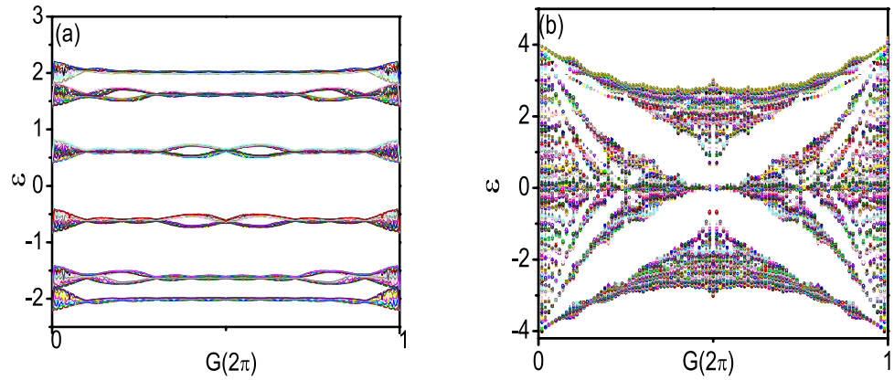
Figure 1. Energy varying with the wave vector G of the FIDSW for (\text{TMTSF})_2\text{X} with t_a/t_b=10 and the FIDSW strength \Delta=0.2 (a), \Delta=2 (b), here t_a=1 is set as the unit of energy 25 .
