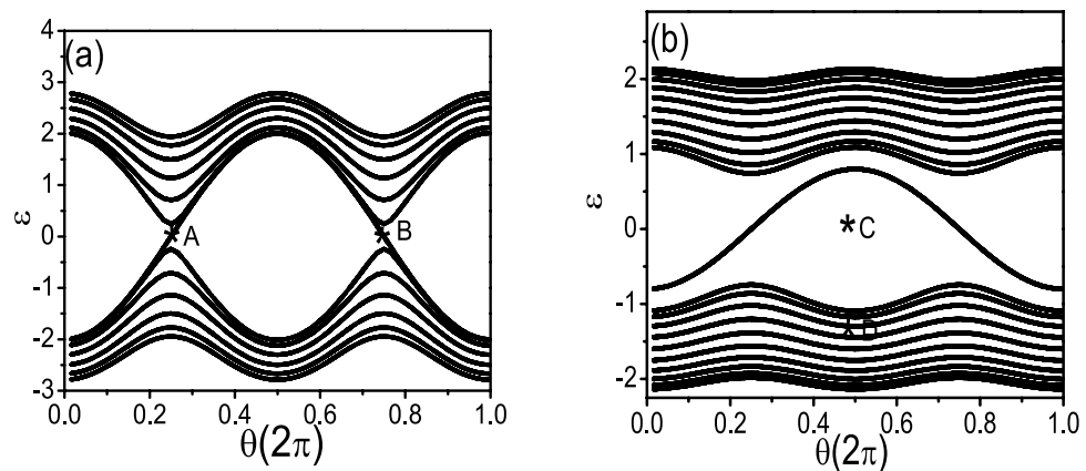
Figure 2. Under open boundary conditions, energy varies with the dimerization effect induced \theta for (\text{TMTSF})_2\text{X} materials with t_a/t_b=10 and the FIDSW strength \Delta=2 , the dimerization strength \delta t=0.1 (a), the FIDSW strength \Delta=0.4 , and the dimerization strength \delta t=0.3 (b).
